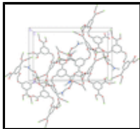
Fig. 2. The perspective view of the polymeric structure. The hydrogen atoms and solvent molecules have been omitted for clarity.
